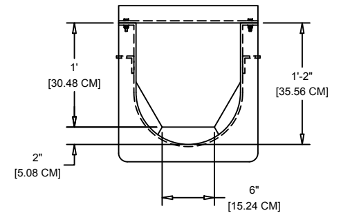
ELEVATION VIEW
