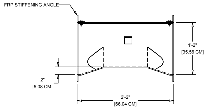
ELEVATION VIEW
