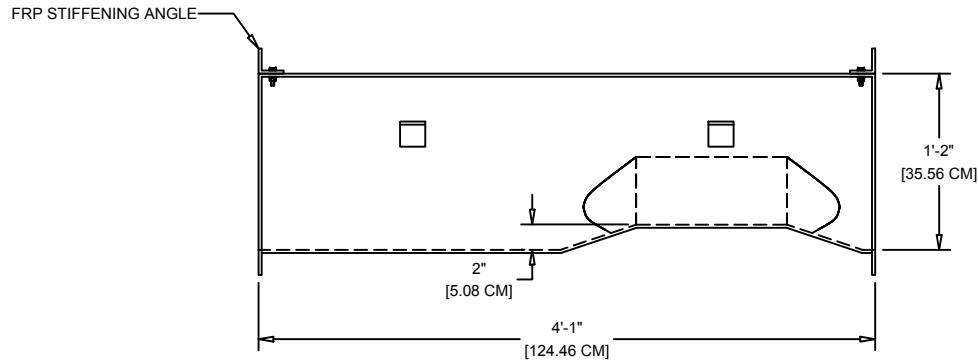
ELEVATION VIEW
