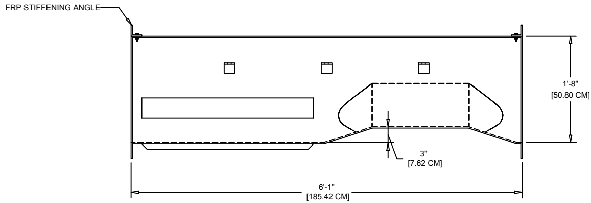
ELEVATION VIEW
