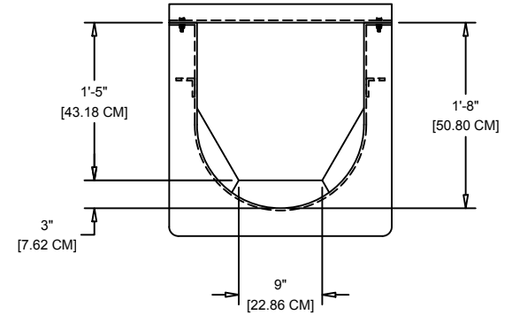
ELEVATION VIEW
