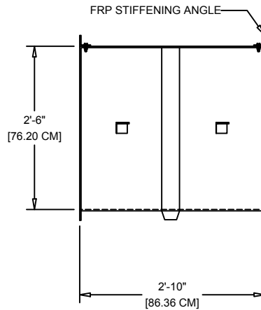
ELEVATION VIEW
